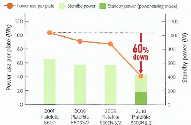
Trends in PlateRite 8600 series electricity consumption (SCREEN measurements)
