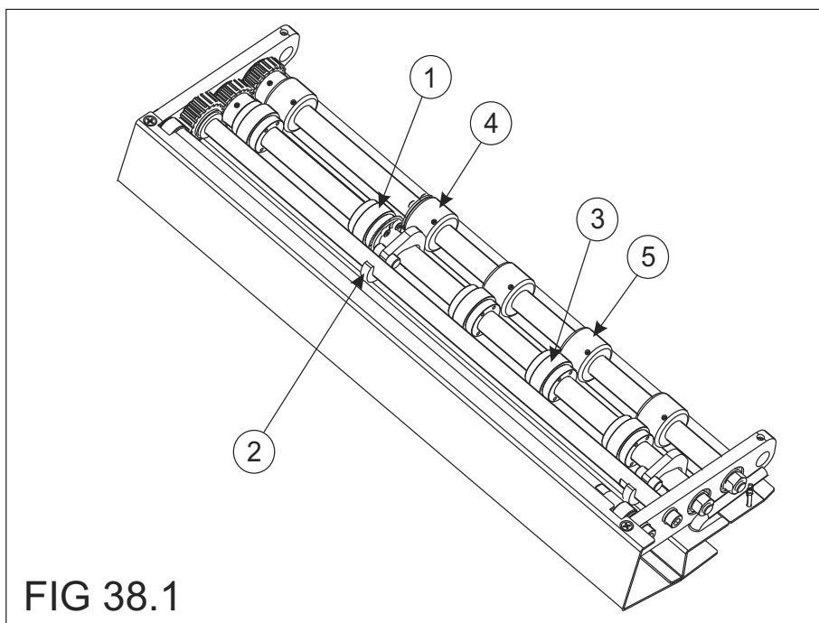
Fig 38.1 Demonstrates a typical set-up for perforating sheets.
