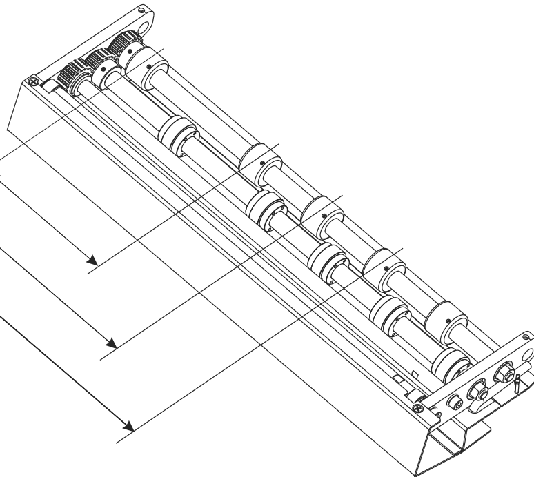
WHEEL & HUB ARRANGEMENT, (WHEN FOLDING)
