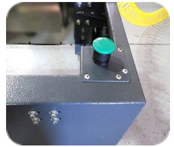
Green switch opens bottom flap folders allowing next box to be placed in machine
