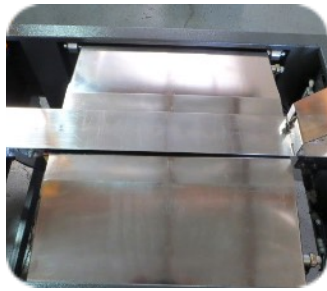
Bottom flap folders in closed position will hold box in place for loading
